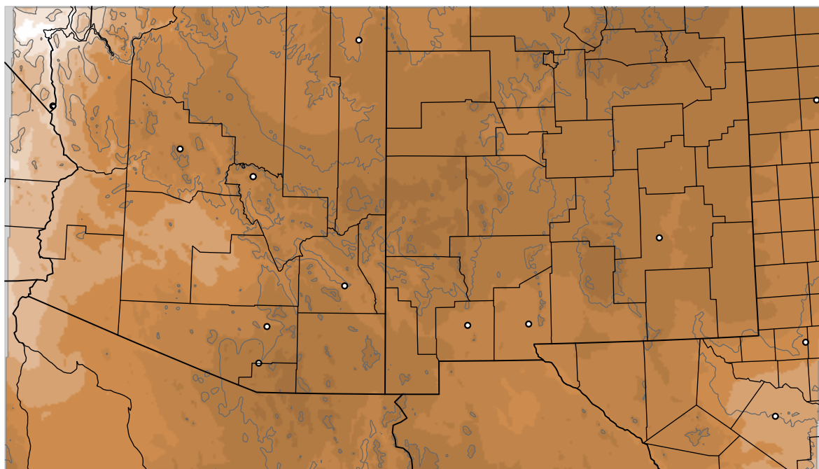
Corrected PWV 9 Jan 2023 14:45 UTC
