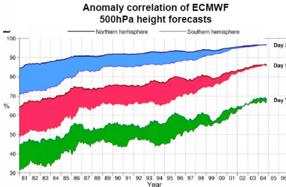
Figure 1. 500 hPa = 500 mb height skill versus time. 500 hPa height is a useful variable with which to evaluate skill because it is tied to the temperature in the lower half of the troposphere and steering winds. See QJRMS 128, p. 652 (2002) ECMWF. From www.bom.gov.au/bmrc/basic/wksp16/pdf_docs/Mon/Simmons_Monday.pdf
