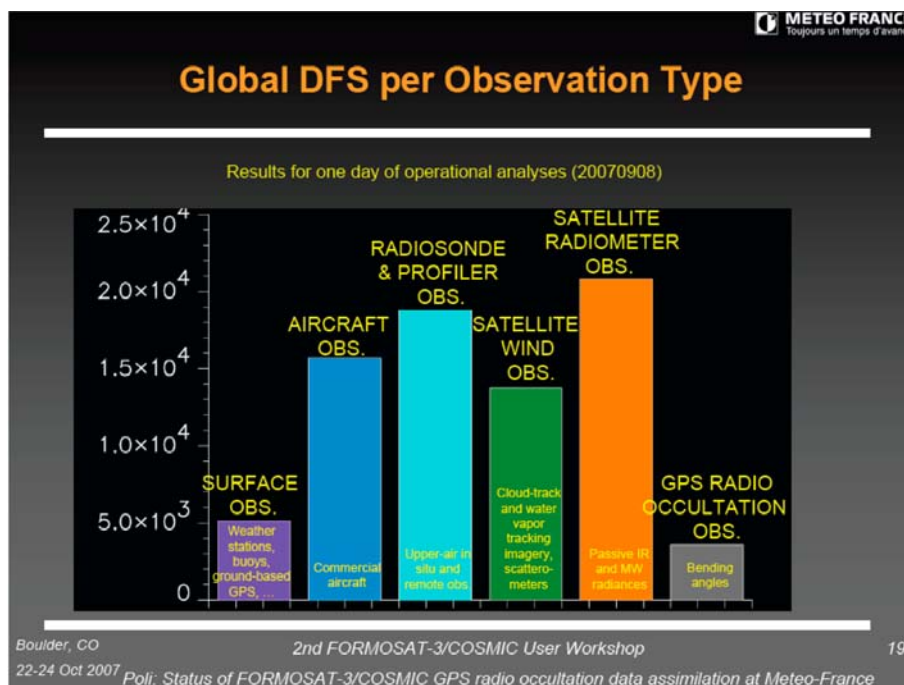
Figure 3. Assessment of the information content and impact of each class of observational data. DFS = “Degrees of Freedom for signal”. From Paul Poli’s presentation at the 2007 COSMIC conference. See http://www.cosmic.ucar.edu/oct2007workshop/program.html .
