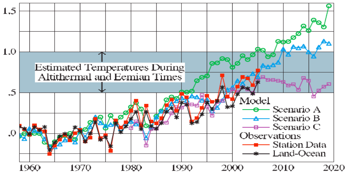
Fig. 2. Global surface temperature computed for scenarios A, B, and C (12), compared with two analyses of observational data. The 0.5°C and 1°C temperature levels, relative to 1951–1980, were estimated (12) to be maximum global temperatures in the Holocene and the prior interglacial period, respectively.
