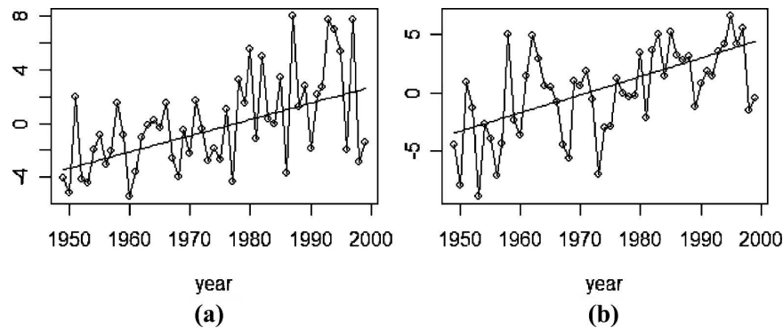
FIG. 2. Time series of PC1 for the Julian day when the (a) 10th and (b) 50th percentiles of the summer (July–September) seasonal rainfall have accumulated. The trend line is the nonparametric Kendall–Theil slope of the data.
