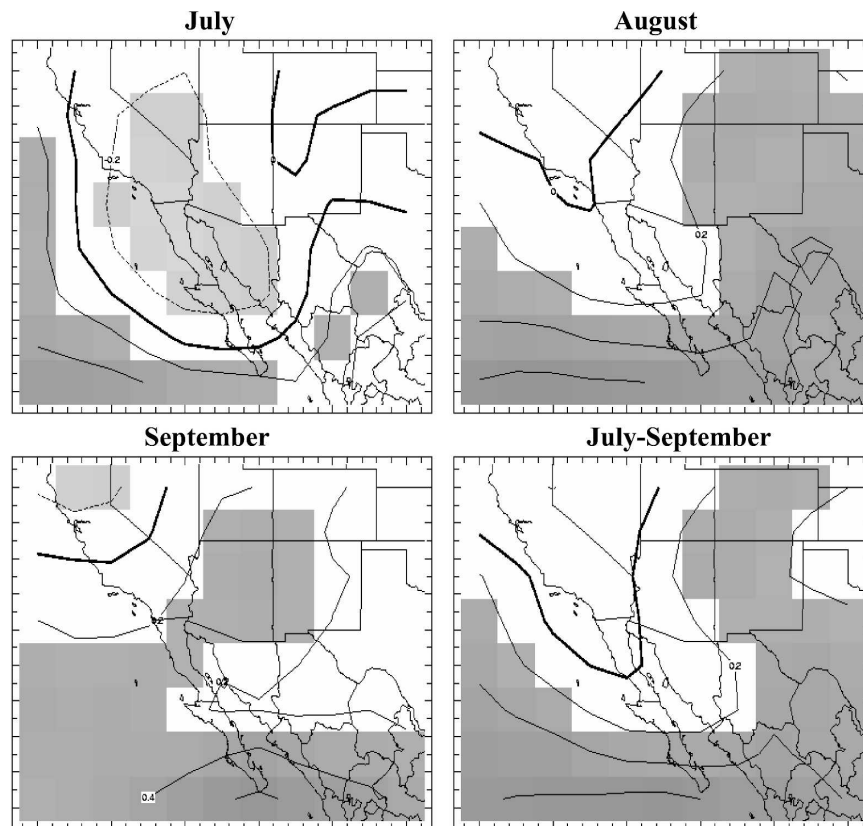
FIG. 5. Trends in monthly and seasonal precipitable water. Shaded regions indicate approximate 90% significance.
