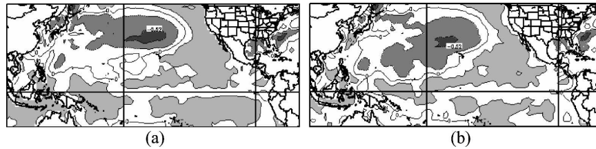
FIG. 9. Correlations between the winter–spring (December–May) SSTs and the first PC of the Julian day of the (a) 50th and (b) 10th percentiles. Correlations above 0.25 and below -0.25 are 90% significant. Shaded regions are statistically significant at the 90% confidence level. (Images provided by the NOAA–CIRES Climate Diagnostics Center, Boulder, CO, from their Web site: http://www.cdc.noaa.gov/ .)
