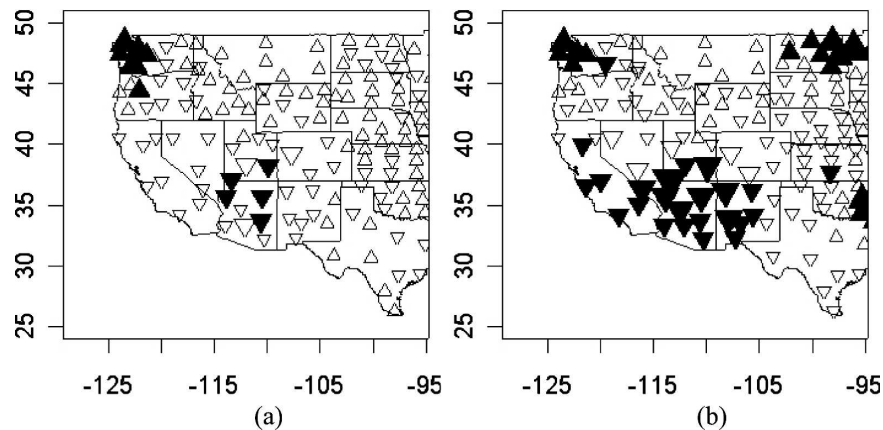
FIG. 8. Correlation map of the rainfall amount's first PC for (a) July–September and (b) July with antecedent winter–spring precipitation. Point-up triangles indicate a positive correlation, and point-down triangles indicate a negative correlation. Symbol size indicates the relative magnitude of the correlation and filled symbols indicate 90% significance.
