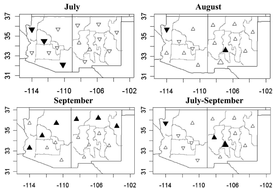
FIG. 4. Trends in summer monthly and seasonal rainfall. Point-up triangles indicate an increasing trend and point-down triangles indicate a decreasing trend. Size indicates the relative magnitude of the trend. For July–September, the triangle sizes correspond to approximately <0.4, 0.4–0.7, and >0.7 in. Filled symbols indicate 90% significance.
