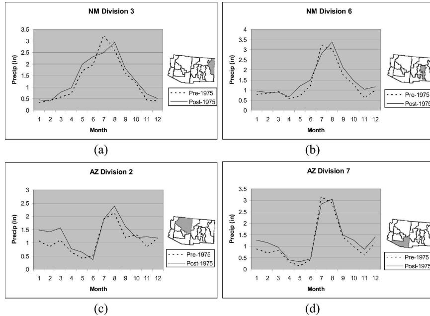
FIG. 3. Annual cycle of precipitation during 1948–75 (dashed line) and 1976–2004 (solid line) at two climate divisions in (a), (b) NM and (c), (d) two climate divisions in AZ.
