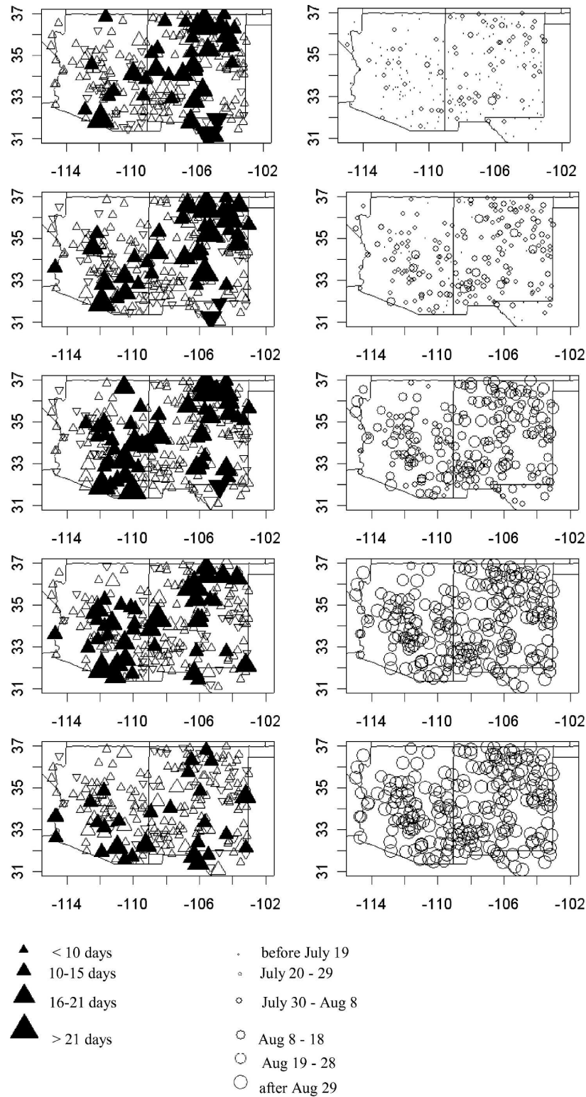
FIG. 1. Trends in Julian day of summer (July–September) seasonal rainfall accumulation at five thresholds (10th, 25th, 50th, 75th, and 90th percentiles; left column, top to bottom, respectively) and the corresponding climatological Julian days (right column, top to bottom, respectively). For the Julian day trends, point-up triangles indicate delay and point-down triangles indicate advancement. Triangle size indicates the magnitude of the trend. Filled triangles indicate 90% significance. For the climatological Julian days, the six circle sizes represent six Julian day windows.
