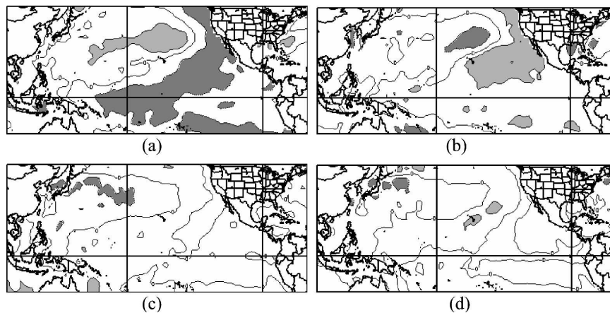
FIG. 10. Same as in Fig. 9 except for correlations between the winter–spring (December–May) SSTs and the first PC of the (a) July, (b) August, (c) September, and (d) July–September monsoon rainfall.
