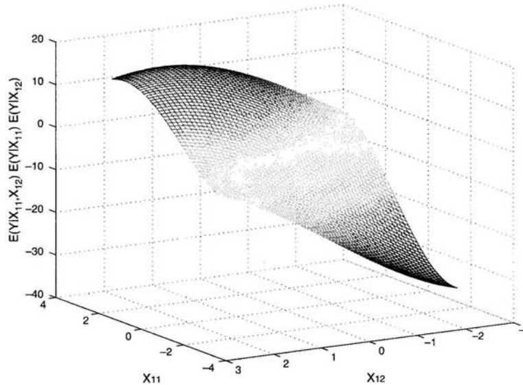
Fig. 2. Posterior expectation of E(Y|x_{11}, x_{12}) - E(Y|x_{11}) - E(Y|x_{12}) against x_{11} and x_{12} : synthetic example
