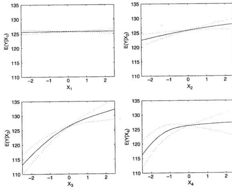
Fig. 4. Posterior expectation of E(Y|x_i) against x_i for four input variables (....., \pm 2 standard deviations): reservoir example
