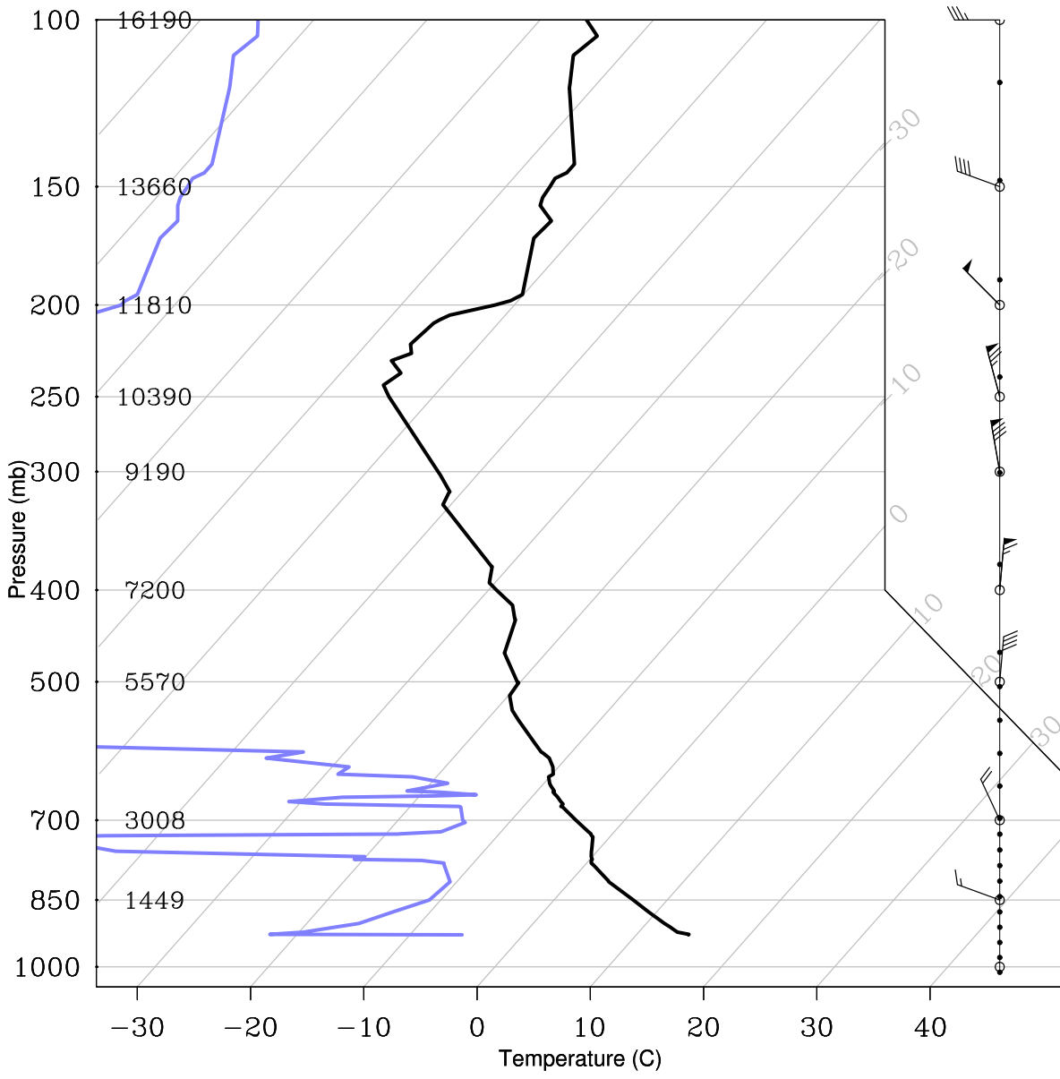
HW3 Skew-T fig2a
