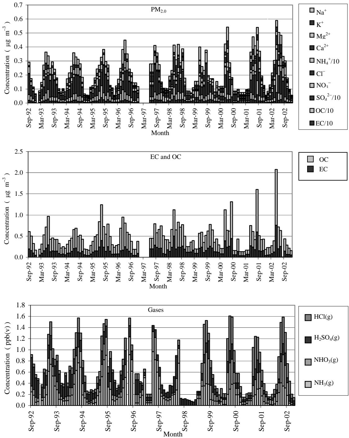
Figure 2. Monthly mean mass concentrations of PM 2.0 , EC and OC and precursor gases. Gaps in data represent months for which data are not available.
