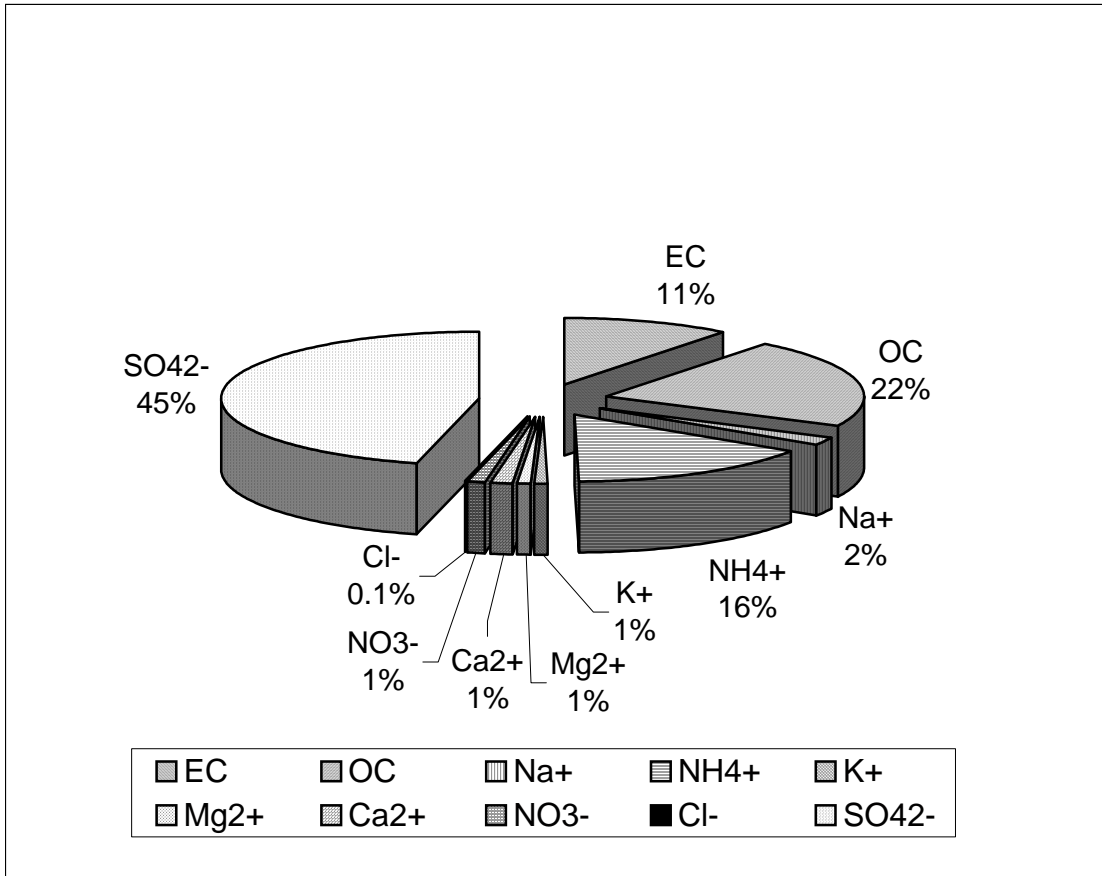
Figure 1. Decade-long mean composition of PM 2.0 from September 1992 to December 2002 in percent by mass ( \mu\text{g m}^{-3} ). Mean total mass is 1.48 \mu\text{g m}^{-3} .
