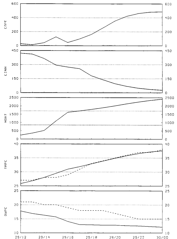
FIG. 8. (top to bottom) Meteorograms of forecast CAPE ( \text{J kg}^{-1} ), CIN ( \text{J kg}^{-1} ), PBL height (m), surface temperature ( ^{\circ}\text{C} ), and surface dewpoint ( ^{\circ}\text{C} ), using the one-dimensional bulk model. The dashed lines in the lower two panels represent the observed temperature and dewpoint, respectively, from nearby Sky Harbor International Airport.
