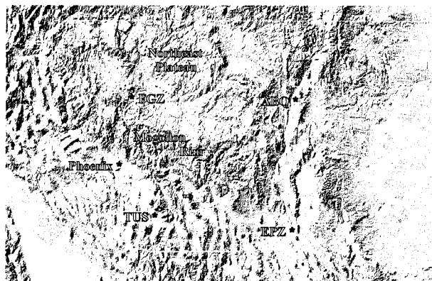
FIG. 1. The topography of the southwest United States. Location of National Weather Service rawinsonde sites Albuquerque, NM (ABQ), Santa Teresa, NM (EPZ), Flagstaff, AZ (FGZ), and Tucson, AZ (TUS) are indicated.
