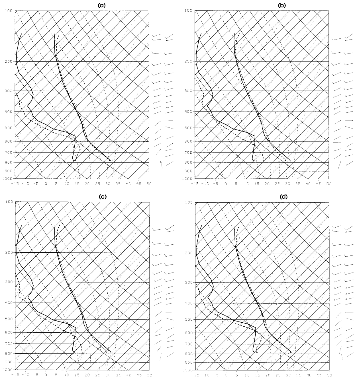
FIG. 12. As in Fig. 11 except for Flagstaff, AZ.
