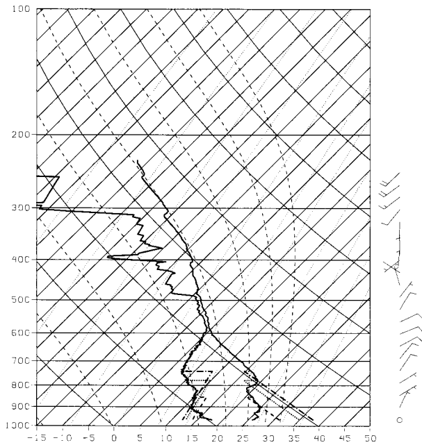
FIG. 7. Skew T -log p plot of sounding at Phoenix, AZ, 1200 UTC 29 Jun 2000 (solid) and PBL forecast sounding valid at 1600, 2000, and 0000 UTC (dash-dot, dot, dash-dot, respectively) using a one-dimensional bulk model. Wind at 1200 UTC in \text{m s}^{-1} .
