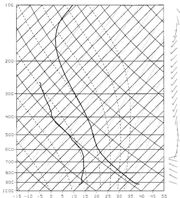
FIG. 4. Skew T -log p plot of 0000 UTC composite sounding for all dry days at Tucson, AZ, between 10 and 19 Jul 1961–90. Wind in \text{m s}^{-1} .
