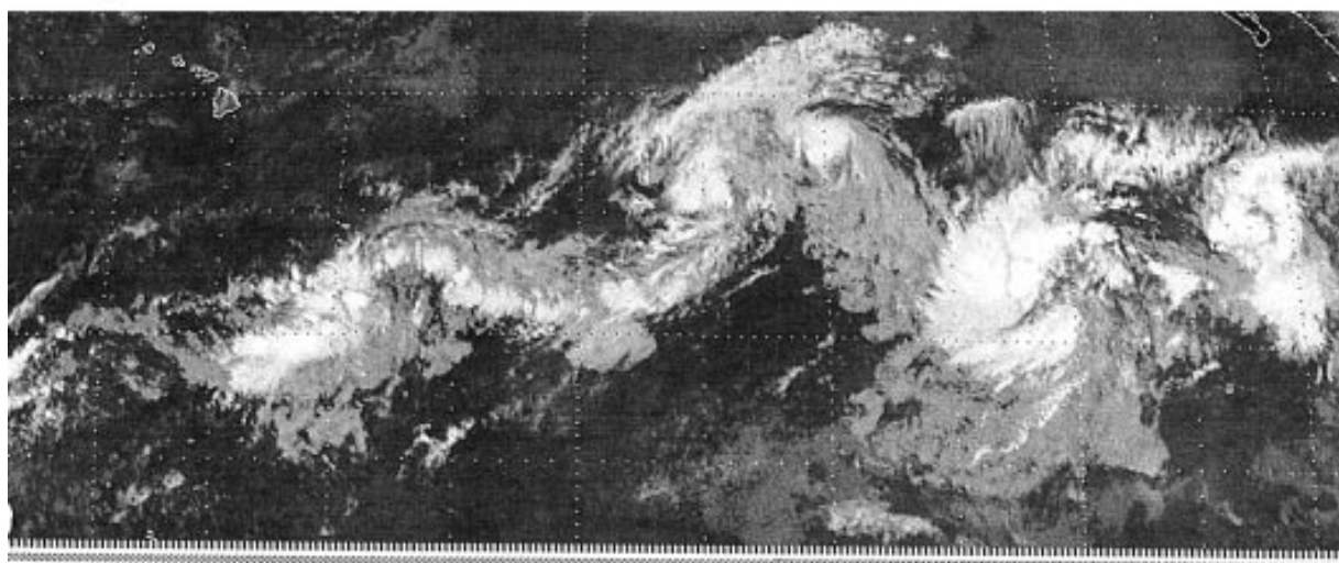
FIG. 1. GOES IR images at 1646 UTC on (a) 26 July, (b) 28 July, (c) 3 August, and (d) 12 August 1988 showing a case of ITCZ breakdown. The images cover a region of the eastern Pacific between 2^{\circ}\text{N} and 24^{\circ}\text{N} , 108^{\circ}\text{W} and 165^{\circ}\text{W} . Hawaii is at the upper left and Baja California at the upper right corners of the images.
