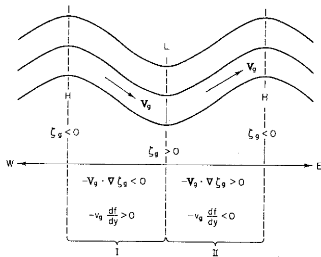
Fig. 6.7 Schematic 500-mb geopotential field showing regions of positive and negative advections of relative and planetary vorticity.
