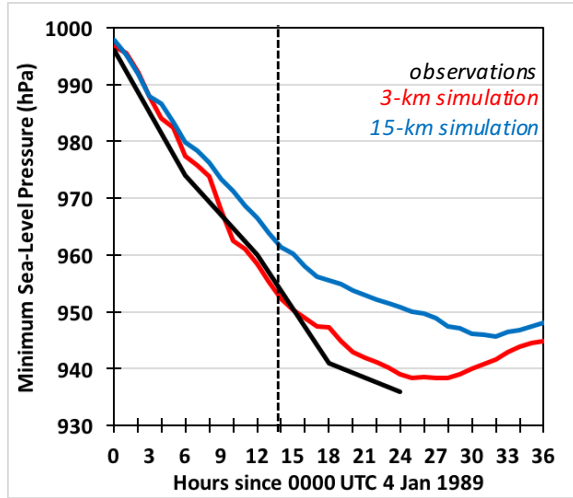
a) cyclone intensity
