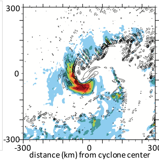
b) cyclone structure (3-km simulation)
