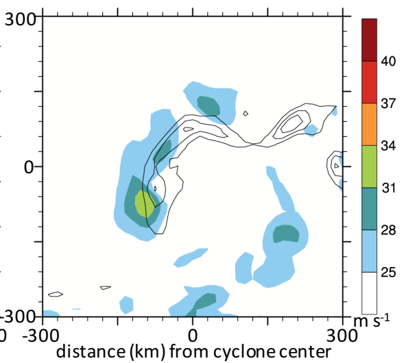
c) cyclone structure (15-km simulation)
